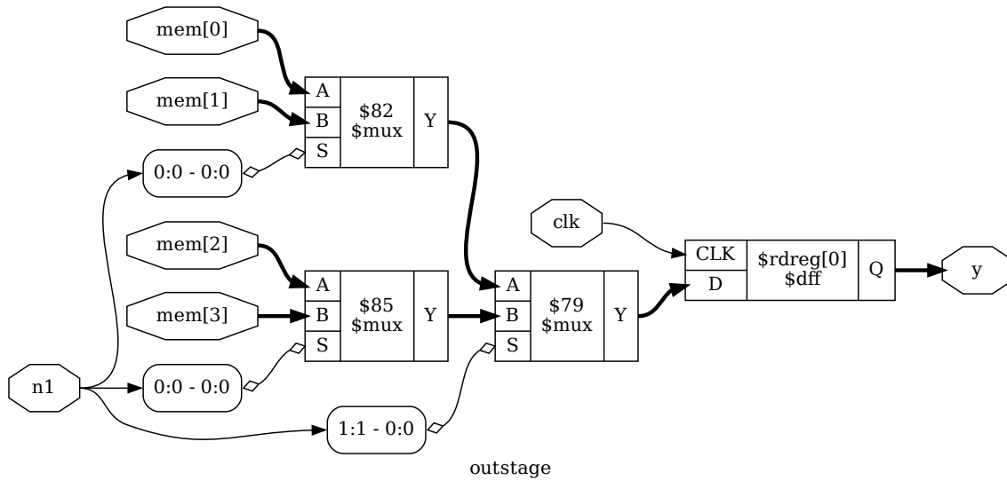
Fig. 3.31: outstage
