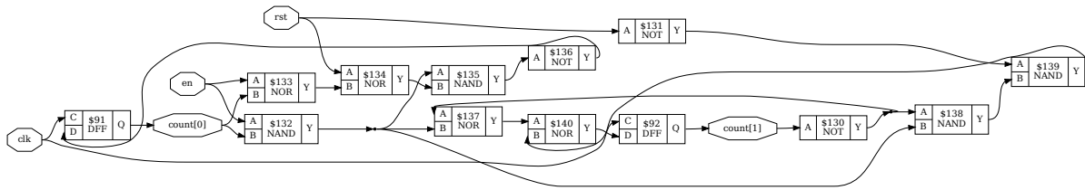
Fig. 3.10: counter after hardware cell mapping
