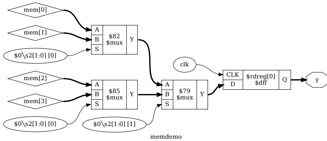
Fig. 3.21: Output of show y %ci2:+$dff[Q,D] %ci*:-$mux[S]:-$dff
